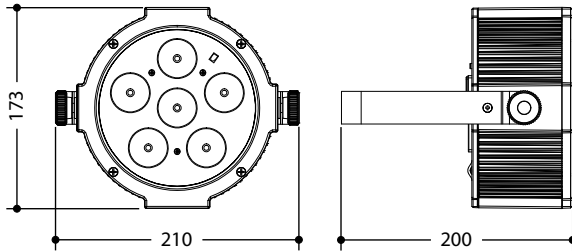
Technical drawing
