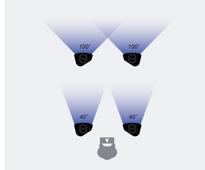
Long Throw System: 2 x P12 + 2 x P12 delayed – all with 'PS horn'
