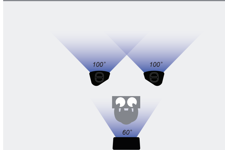
Small Club: 2 x P12 with 'PS Horn' for FOH, 1 x P12 with standard horn for monitor
